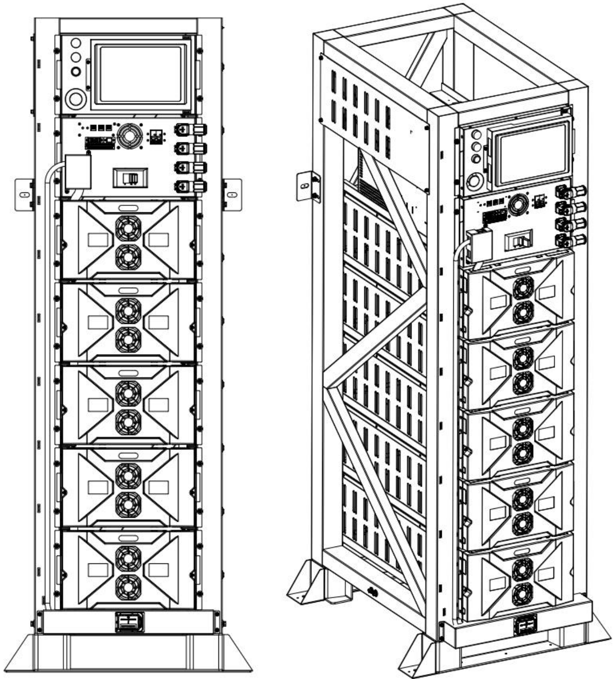
Figure 3.4.4 Product Layout Diagram of 5 PACK (with a capacity of 100kWh)
