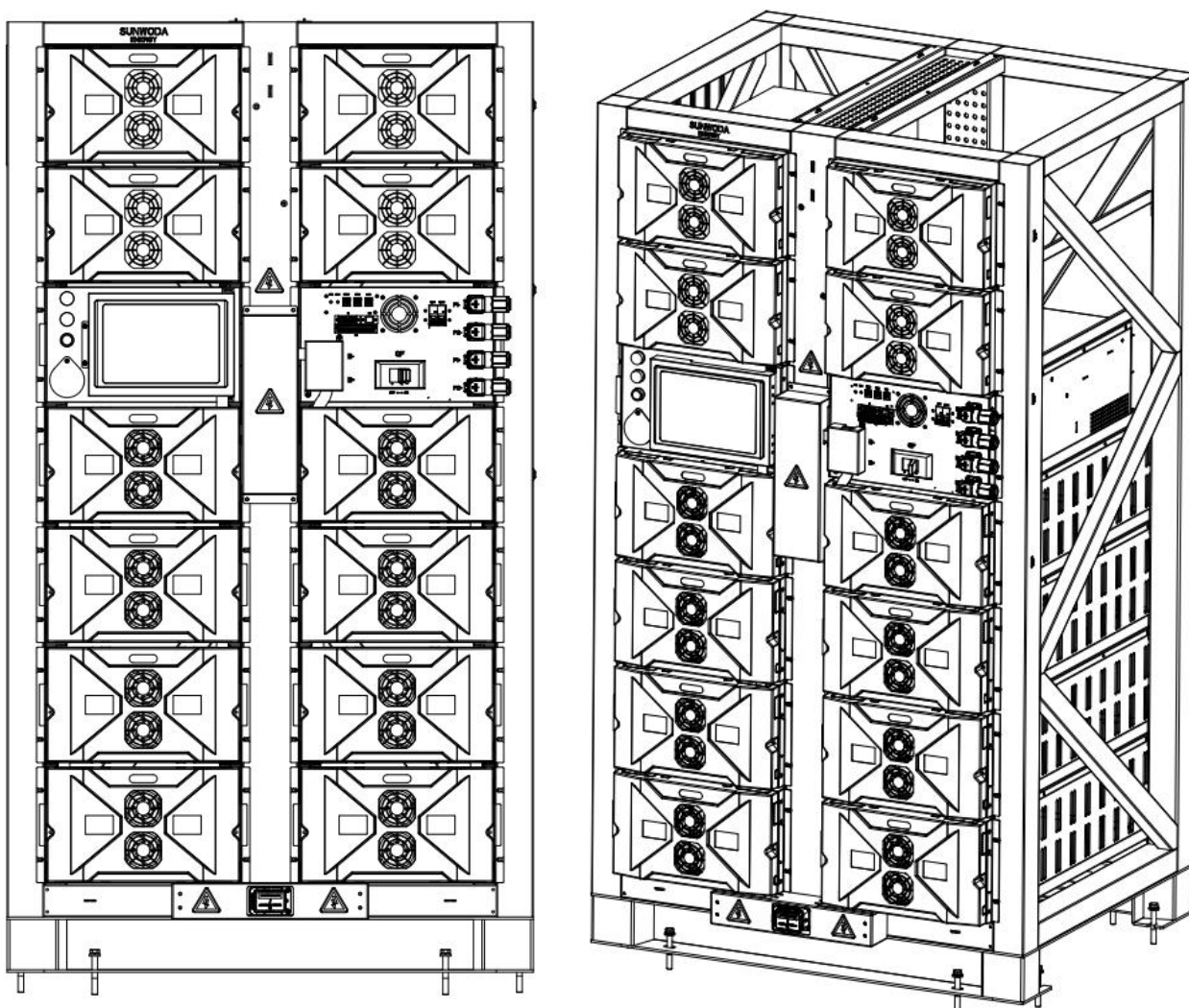
Figure 3.4.3 Product Layout Diagram of 6 to 8 PACK (with a capacity of 120~160kWh)
